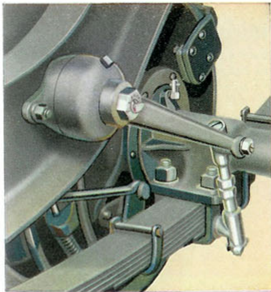
Double action Houdaille hydraulic shock absorbers with an exclusive Nash design outboard mounting enhance the luxury of riding in the Advanced Six models
