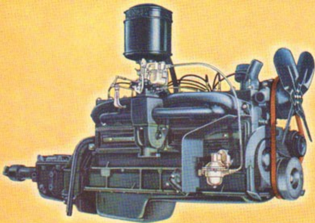
Packard Eight Clipper Engine for 1946
