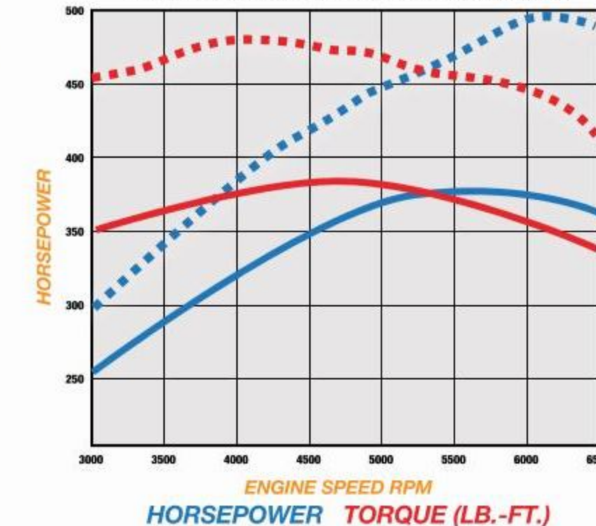
2018 500HP 5.3L SPORT EDITION SUPERCHARGED SILVERADO FLYWHEEL HORSEPOWER and TORQUE (lb.-ft.)
