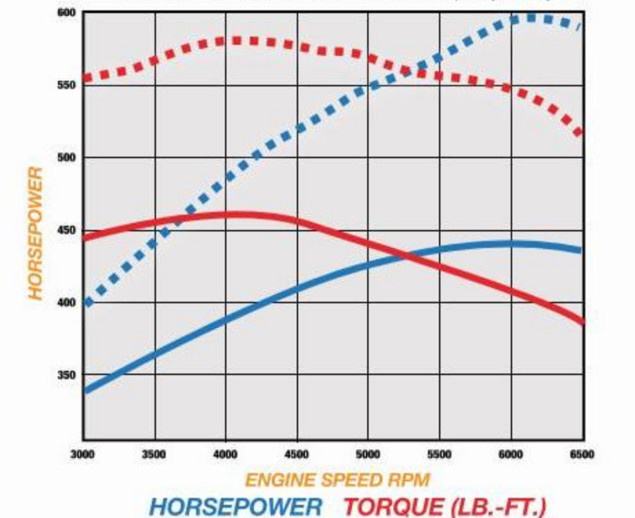
2018 575HP 6.2L SPORT EDITION SUPERCHARGED SILVERADO FLYWHEEL HORSEPOWER and TORQUE (lb.-ft.)
