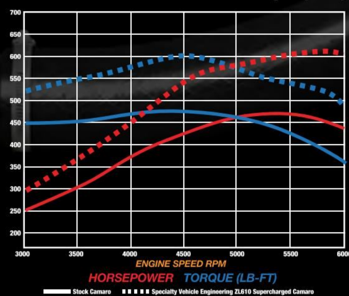
SUPERCHARGED 2018 6.2L V8 CAMARO FLYWHEEL HORSEPOWER and TORQUE (lb-ft)
