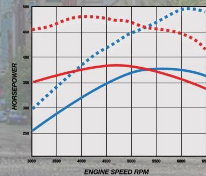
2018 500HP 5.3L SPORT EDITION SUPERCHARGED YUKON FLYWHEEL HORSEPOWER and TORQUE (lb.-ft.)
