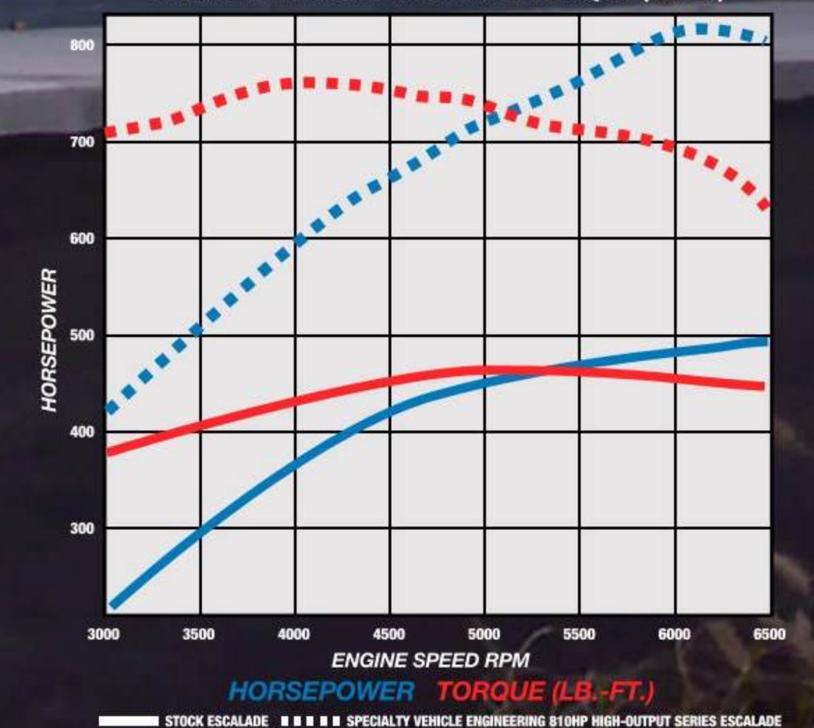
2019 810HP 6.8L HIGH/OUTPUT SERIES ESCALADE FLYWHEEL HORSEPOWER and TORQUE (lb.-ft.)
