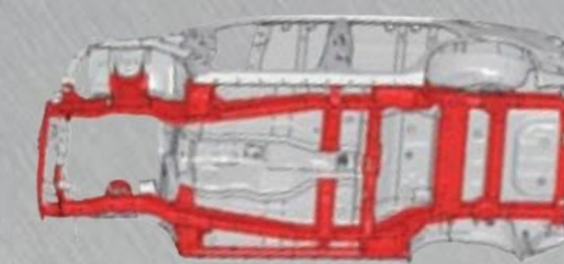
LADDER-FRAME-REINFORCED UNIBODY CONSTRUCTION
