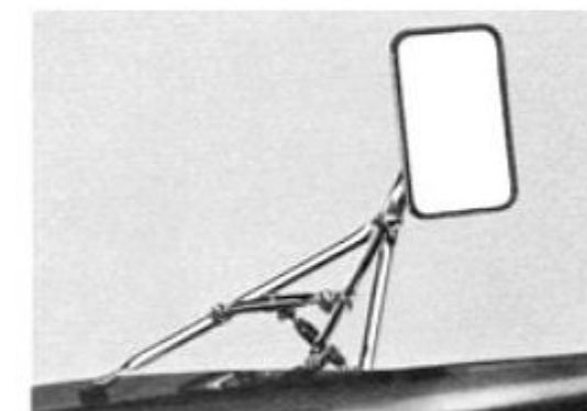
Trailer Towing Mirrors A pair—both right-hand and left-hand. These mirrors are specially designed to fit any Pontiac model. Easy to attach and remove when not in use. Turnbuckle-type fender mounts attach to front wheel opening and held firmly in place when hood is locked. Large 5 1/2" x 8" size. Stainless steel construction. (D)
