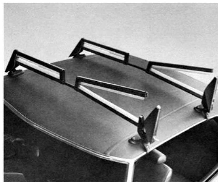
Removable Ski Rack Quickly fastens to roof drip moldings. Features adjustable rubber-padded metal tapes to protect car finish, rubber-padded cross members to protect skis, pushbutton release arms. Everything locks securely to guard against theft. As many as eight pairs of skis can be accommodated at one time. (D)
