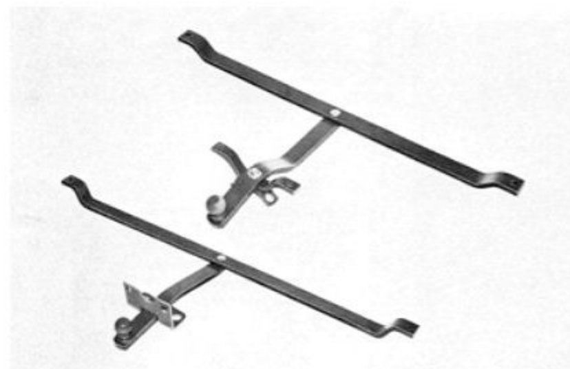
Trailer Hitch (Class I—Light Trailers from 1000 to 2000 lbs. loaded—tongue load up to 200 lbs.) Custom designed for Pontiac vehicles. Chrome plated draw bar and ball. Permanently bolted to structural members of the car. Recommended
