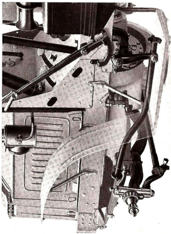
Front Axle and Chassis Parts
