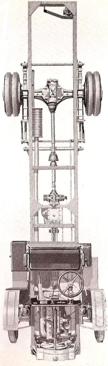
Plan View Standard 5-E Chassis
