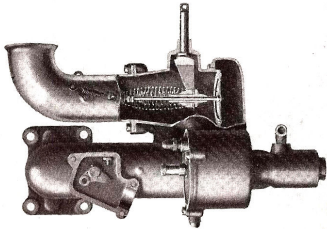
Section Through Air Valve
