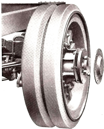
Rear Wheel Drive Universal Joint Action Eliminates Bending Stresses
