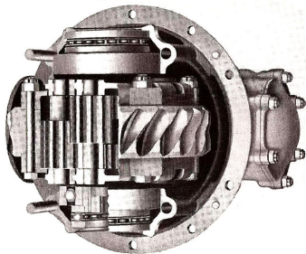
Differential and Carrier
