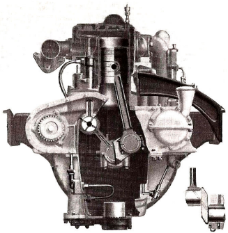
Motor—Cross Section Showing Lubrication System
