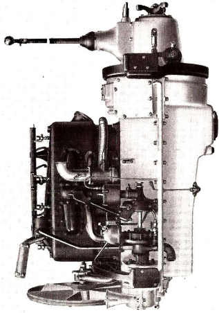
Motor—Left Side Unit Power Plant Contains Motor Clutch and Transmission
