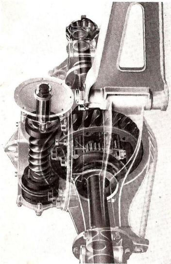
Rear Axle Showing Mounting of Worm and Wheel, Differential Gear and Driving Shafts
