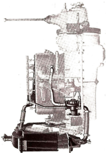
Cooling System Showing Section Through Radiator and Thermostat
