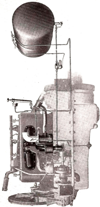
Pressure Feed Gasoline System
