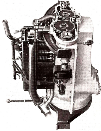
Motor—Right Side Showing Section through Cylinder with Gear Case and Valve Cover Removed
