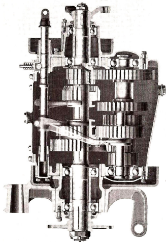
Transmission Four-Speed Selective Sliding Type
