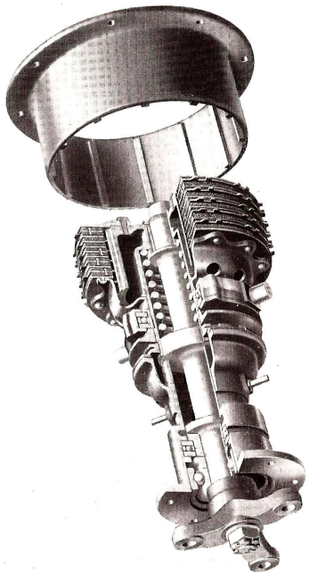
Clutch Multiple Disc Dry Plate Type
