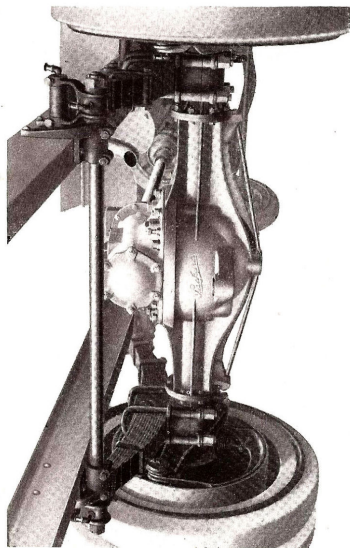
Rear Axle Showing Oil Filler, Rear Spring Trunnions and Mounting of Differential Carrier
