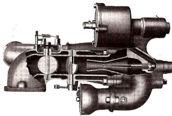
Carburetor Section Through Mixing Chamber
