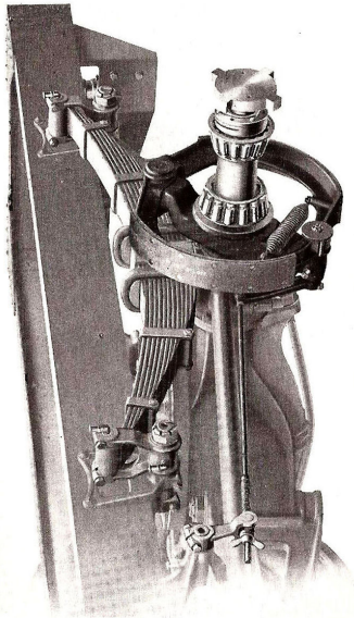
Rear Axle with Wheel Removed Showing Radius Rods, Emergency Brake, Hub End of Axle Shaft and Rear Spring Suspension
