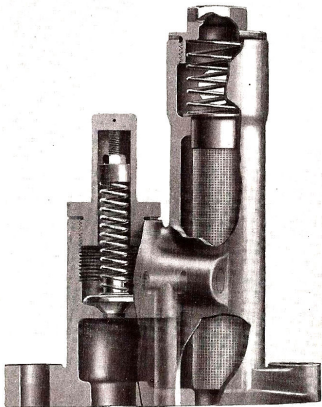
Oil Pressure and Relief Valve
