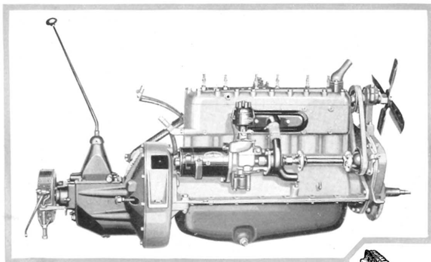
The Dictator Motor 70 Horsepower — 65 Miles per Hour
