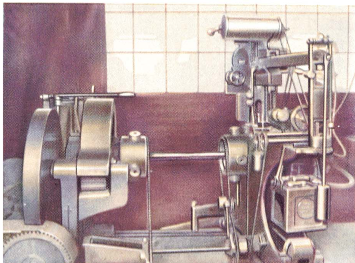
Here, a Studebaker rear axle is being subjected to a laboratory test far more strenuous than will ever be encountered in actual use—a 33,000 inch-pound twist administered by a powerful machine. Axles are chosen at random and subjected to this test to make sure that they measure up to Studebaker's high standards.
