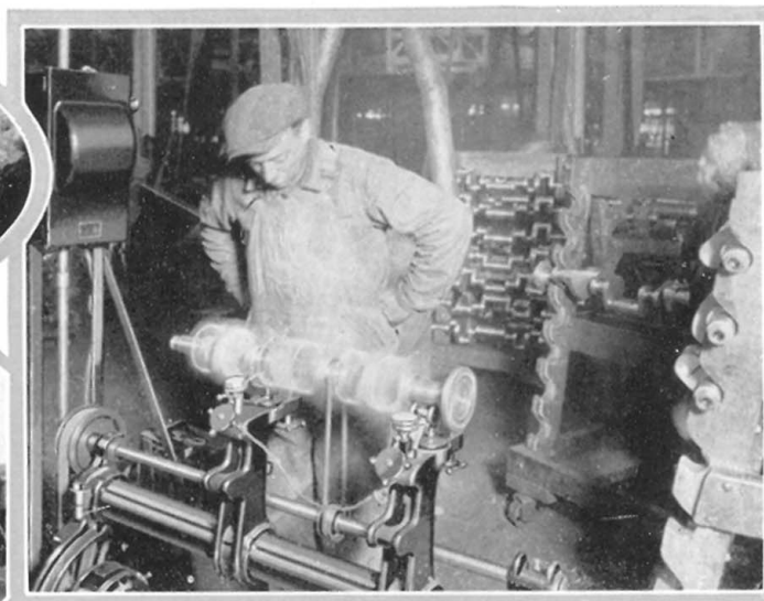
The perfect balance of every Studebaker crankshaft is maintained by constant tests during manufacture. Delicate gauges register any defect while the shaft turns at high speed in this test.
