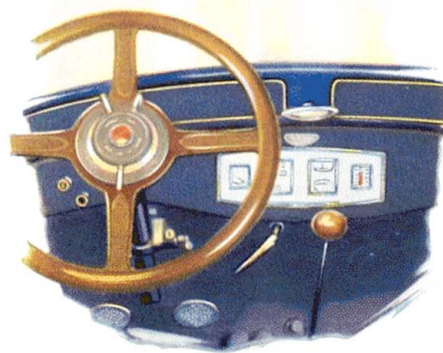
Hydrostatic gasoline gauge, engine thermometer and other indicators all under glass, indirectly illuminated. Twin-beam driving lights controlled from new flat-type steering wheel. No-draft ventilating windshield adjusted from dash. Coincidental lock to steering-ignition mounted at dash.
