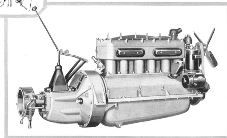
The World's Champion Commander Motor 85 Horsepower—72 Miles per Hour
