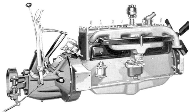
The President Straight Eight Motor 100 Horsepower — 80 Miles per Hour
