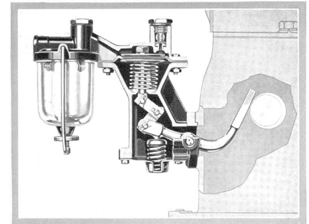
Gasoline is supplied to the carburetor by an automatic fuel pump operated by the cam shaft. Simplicity and reliability dictated its adoption for Studebaker motors. It provides an even flow of gasoline regardless of grade conditions or speed.
