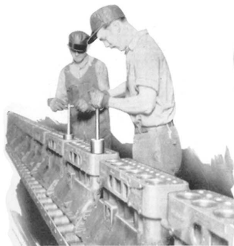
(LEFT) To assure a perfect fit of all pistons, each cylinder is gauged in size down to 1/1000 of an inch and pistons are selected for proper fit of each cylinder. The result is smoother performance.
