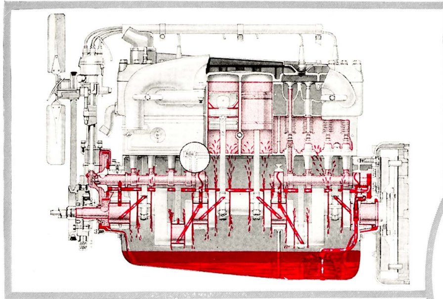
Studebaker's positive force feed lubricating system pumps an ample supply of oil to every part of the motor. Due to advanced design, engine oil need be changed only every 2,500 miles. High pressure chassis lubrication is furnished by magazine lubricators (right) which supply lubricant under pressure and require attention only at 2,500-mile intervals.
