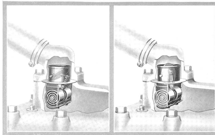
(ABOVE LEFT) Circulation of water is retarded by a valve (operated by coils of a thermostat) until a predetermined temperature is reached. (ABOVE RIGHT) The thermostat then opens valve permitting water to start circulating. This thermostatic control of all Studebaker cooling promotes quick warming of motor in cold weather.
