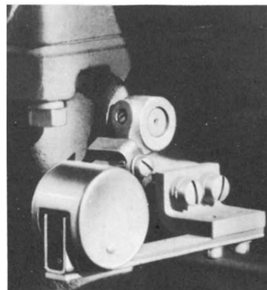
Automatic Heat Control insures efficient motor operation under all conditions by regulating the passage of heat through the exhaust line. In combination with the new downdraft carburetors and automatic choke control it gives to Studebaker cars the finest system of carburetion available today.
