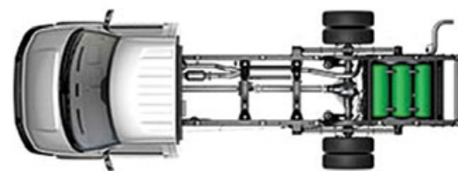
UFM Three-tank system
