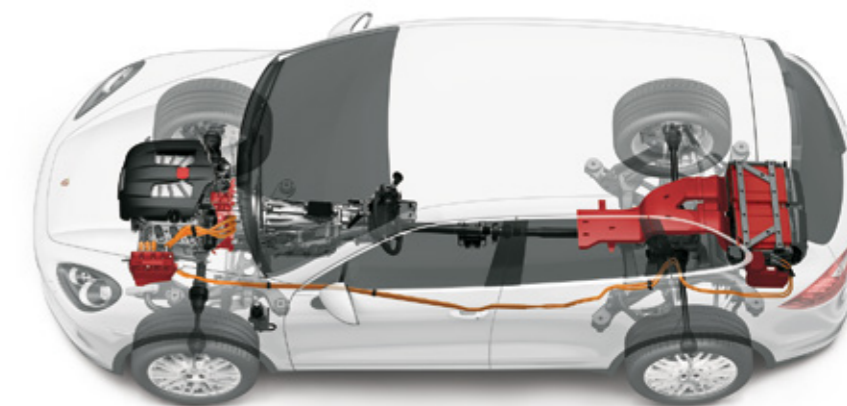
Parallel full hybrid
