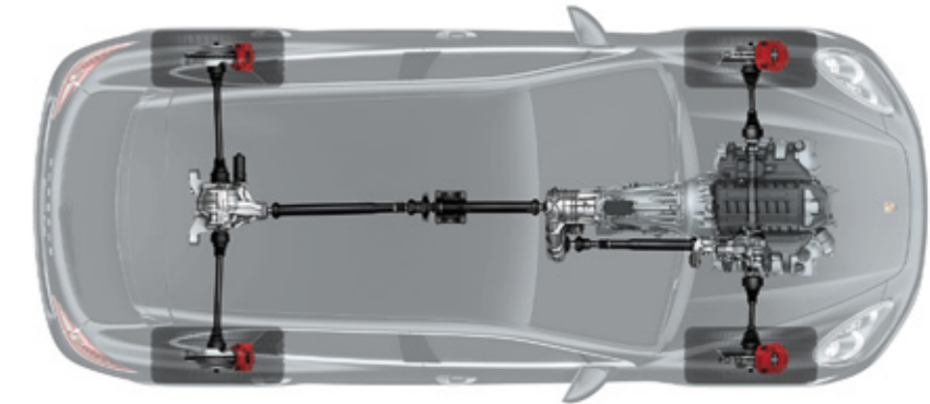
All-wheel drive on the Cayenne, Cayenne S, Cayenne GTS and Cayenne Turbo
