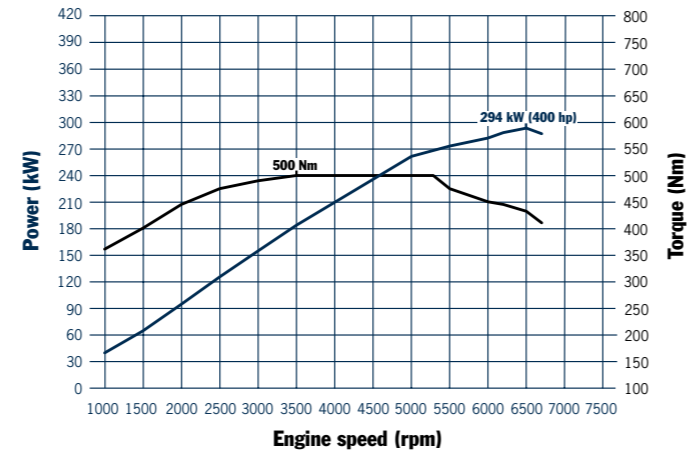
Cayenne S: 500 Nm between 3,500 and 5,300 rpm, 294 kW (400 hp) at 6,500 rpm
