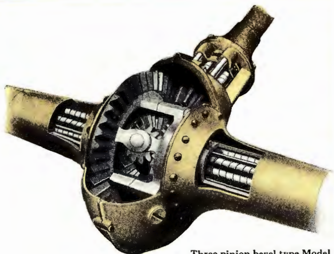
Three pinion bevel type Model T Differential, noted the world over for its simplicity and smooth running
