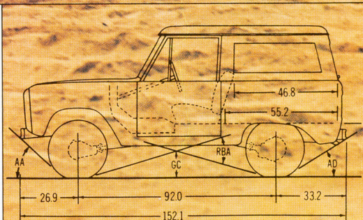
Ground clearance angles and dimensions
