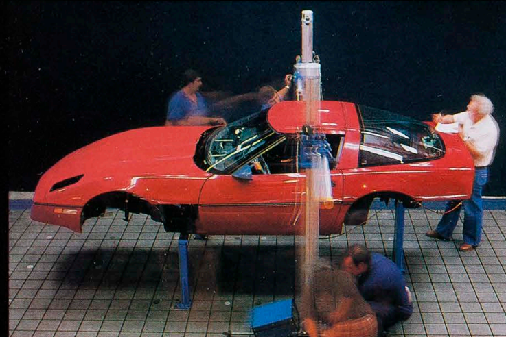
Point-check inspection to make sure body panel assembly meets design intent.
