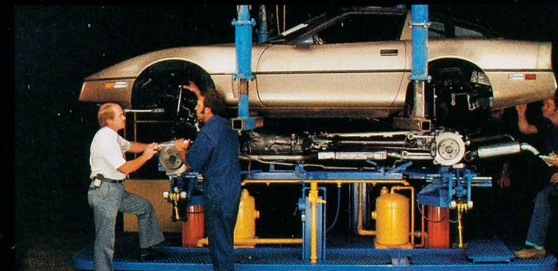
Specially built hydraulic towveyer system "marries" chassis to body.
