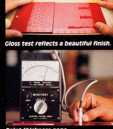
Paint-thickness gage.
