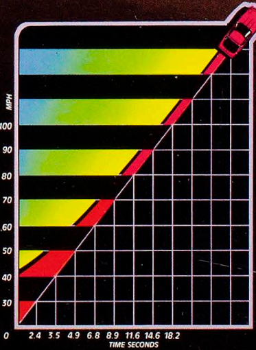
Acceleration 4-speed Automatic/opt. 3.31 Axle
