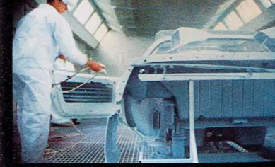
Clean-room environment is a key part of the paint process.
