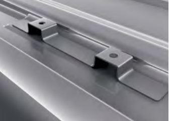
Integrated roof rack-mounting points help secure racks and help reduce likelihood of rusting caused by drilling into sheet metal.
