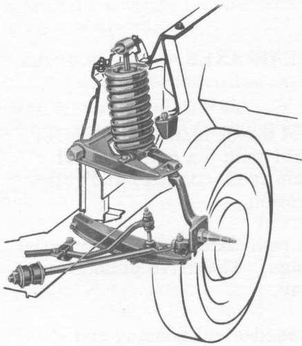
FRONT SUSPENSION
