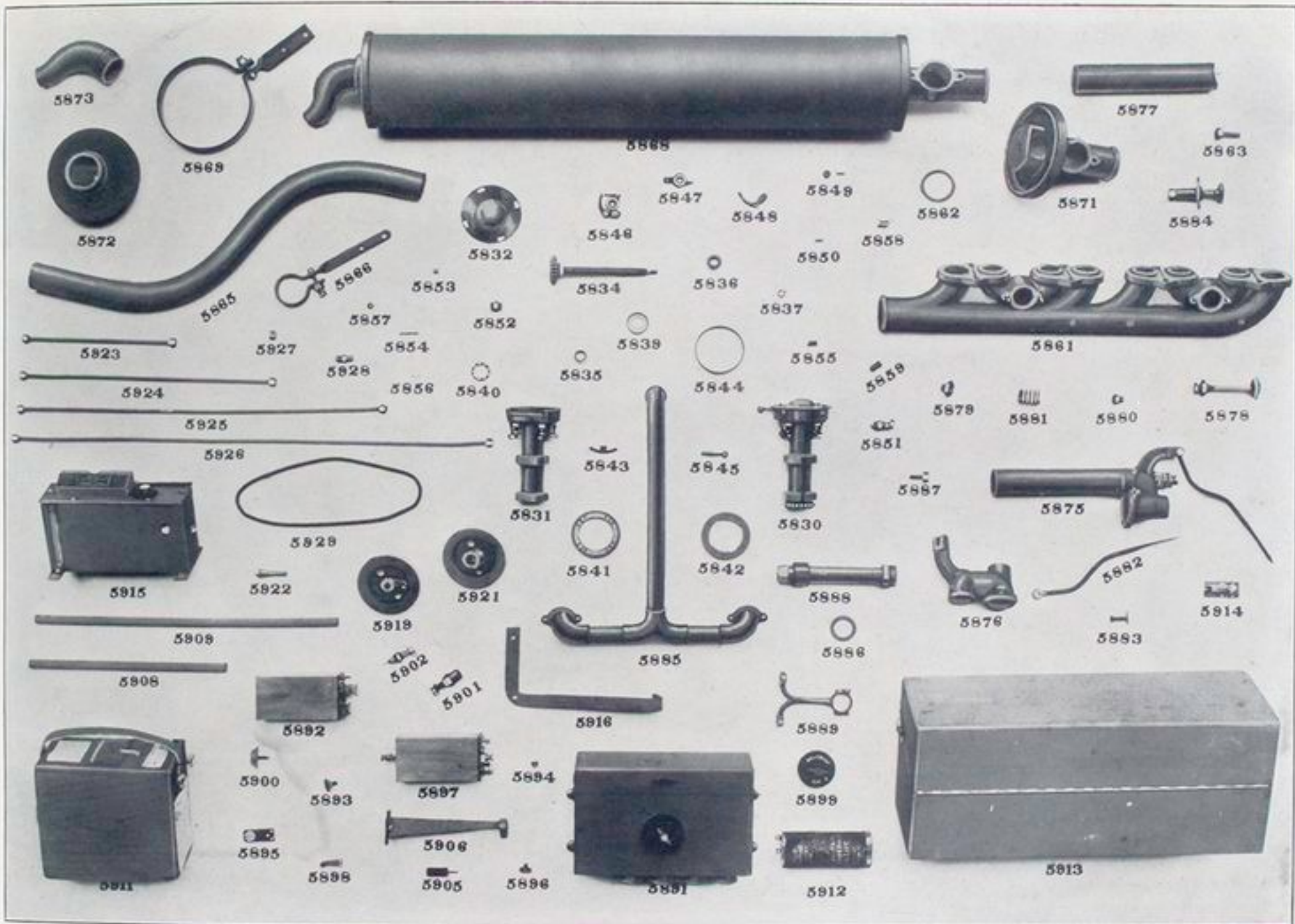
Group 56—Models 34 and 34A
