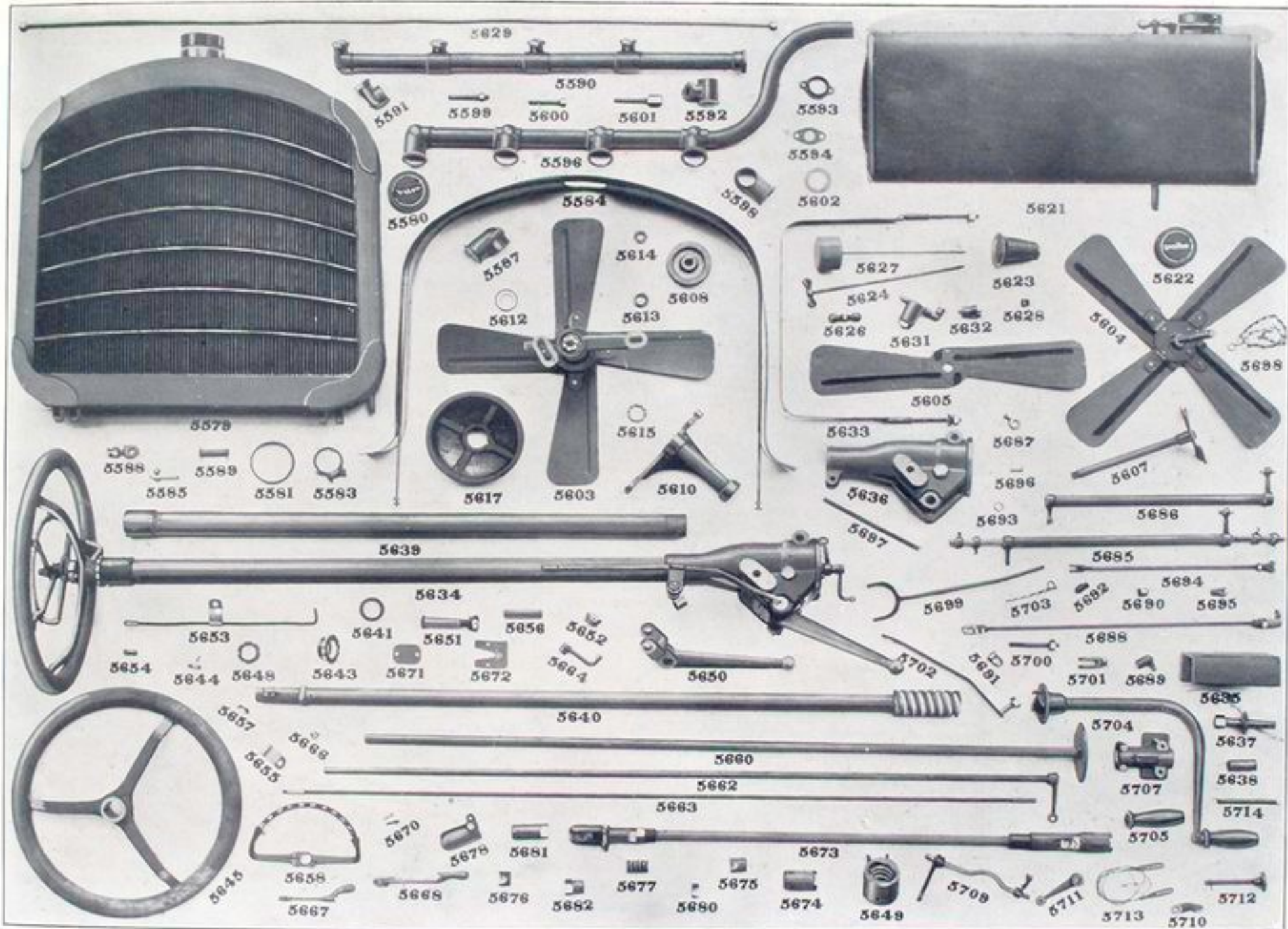
Group 54—Models 34 and 34A
