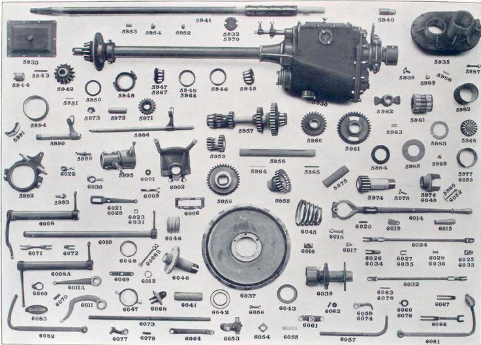
Group 57—Models 34 and 34A
