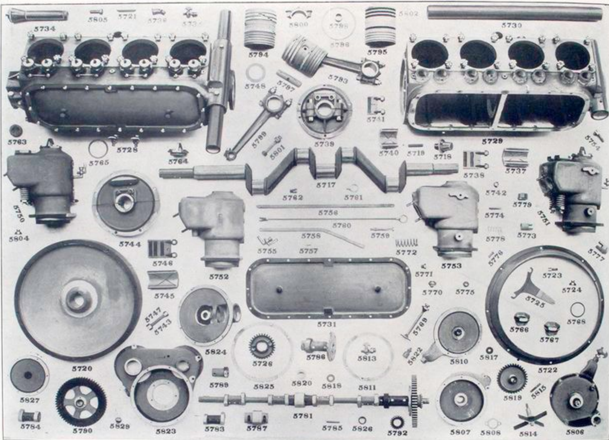
Group 55—Models 34 and 34A
