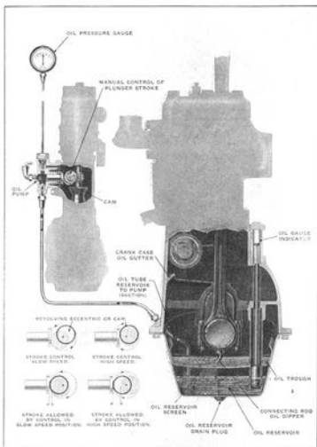
Details of Oiling System
