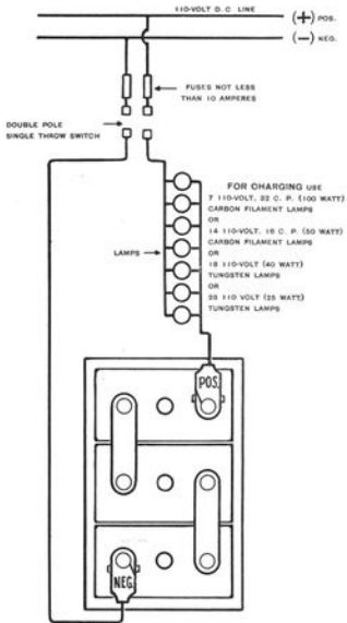
Charging Circuit Diagram
