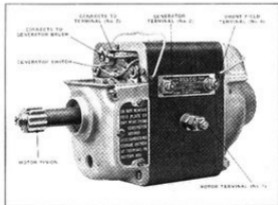
Side View of Generator
