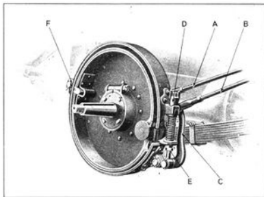
Brake Adjustment
