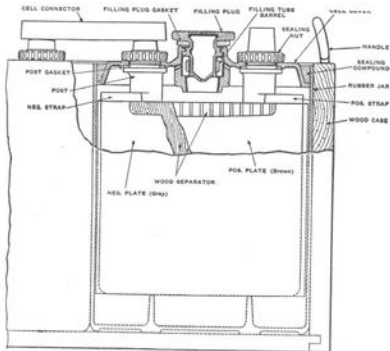
Storage Battery
