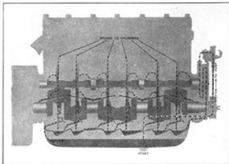
System Diagram
