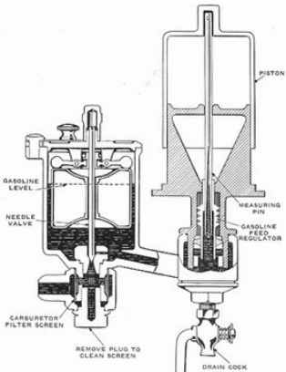
Carburetor Gasoline Level
