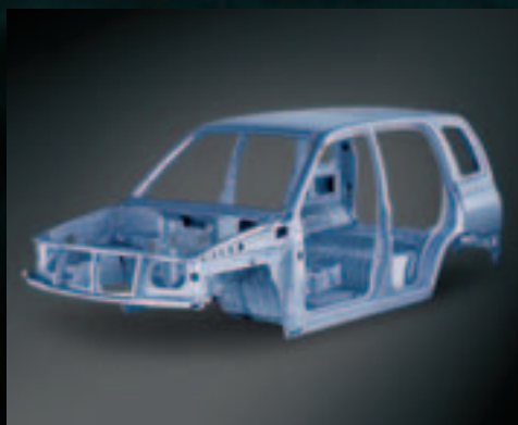
Safety-cage construction — designed to help maintain passenger space in event of collision.
