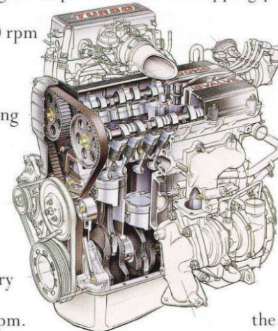
1.6 litre DOHC 16 valve, intercooled turbocharged engine.
