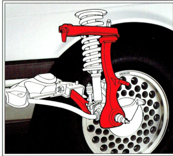
SLALS front suspension system.
