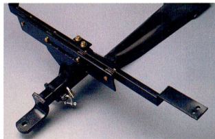
Renowned Hayman Reese towbar.
