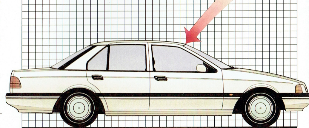
Epoxy resin reinforcement of A and B pillars plus thicker front and side glass has strengthened the passenger compartment.
