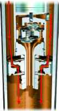
Rebound in 'Sport' mode – damper piston with bypass valve closed
