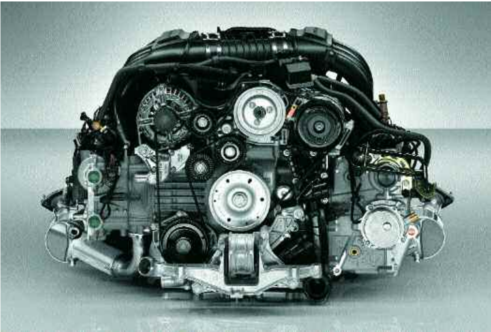
Cayman S: 3.4-litre six-cylinder boxer engine
