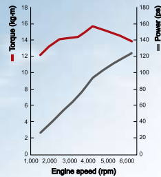
1.6 DOHC CVVT Gasoline Engine
