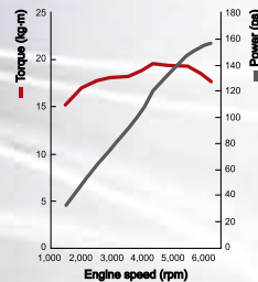
2.0 DOHC CVVT Gasoline Engine
