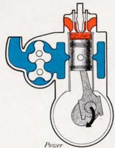
Power
