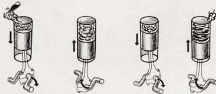
INTAKE
