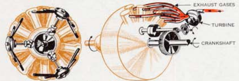
Turbo-compound engine
