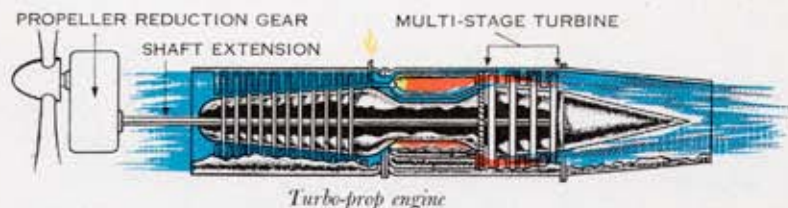
Turbo-prop engine
