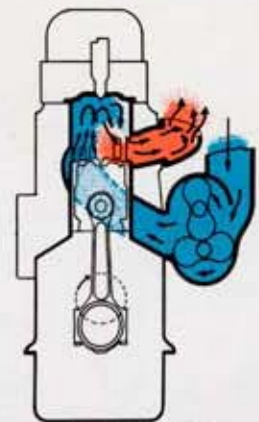
Loop scavenged engine
