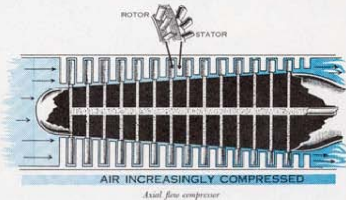
Axial flow compressor
