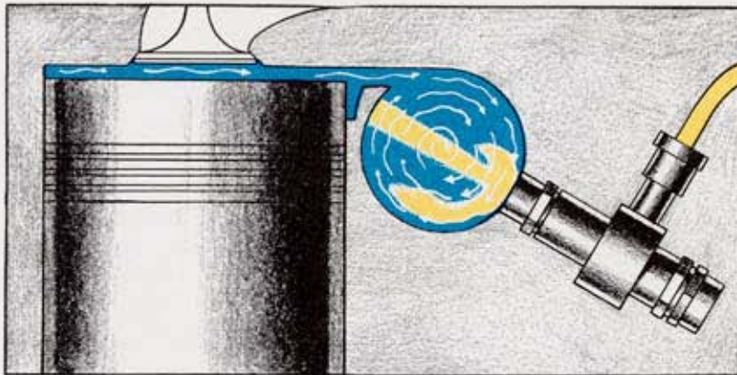
Pre-combustion chamber
