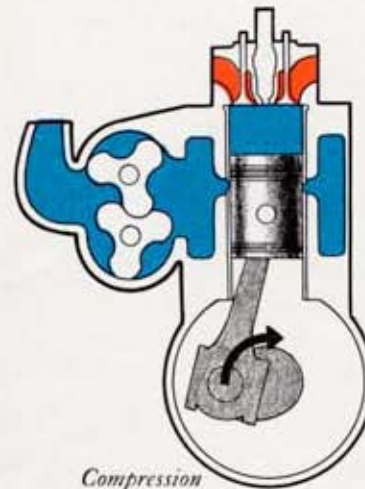
Compression
