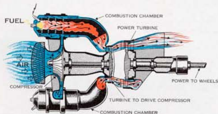
Automotive gas turbine
