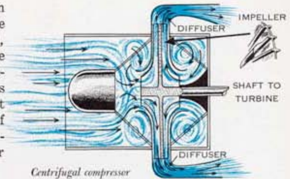
Centrifugal compressor
