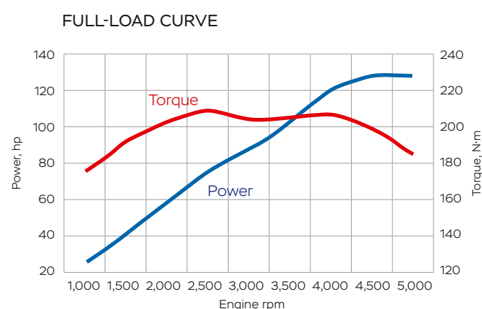
2.7 L 135 hp gasoline engine
