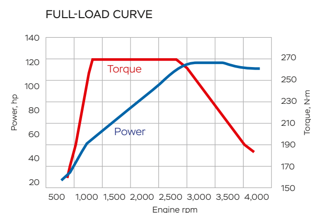
2.2 L 114 hp diesel engine
