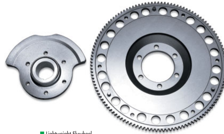
■ Lightweight Flywheel Allows the engine to rev quicker. Manual transmission only. Weight: 6.92kg. Lightweight Flywheel . . . . . QSEA-11-500
