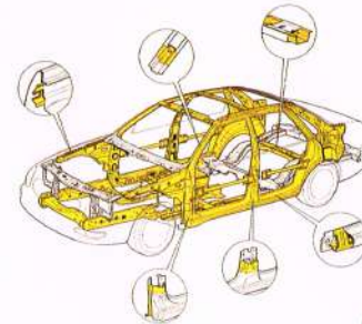
The body structure of the Scorpio forms a high-strength safety cage around the occupants. Includes side impact beams.
