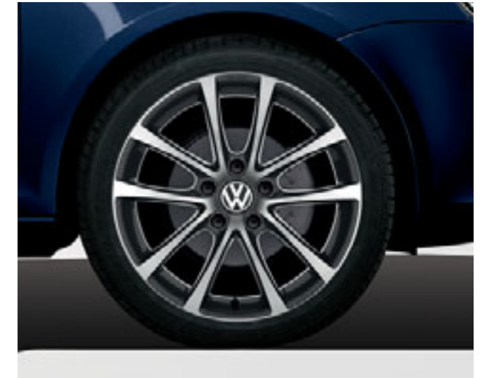
Volkswagen Genuine Azuro alloy wheel Wheel size: 7.5 J x 17" Tyre size: 235/45 R17
