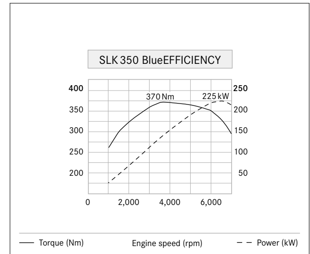
The SLK 350 BlueEFFICIENCY features a state-of-the-art direct petrol injection V6
