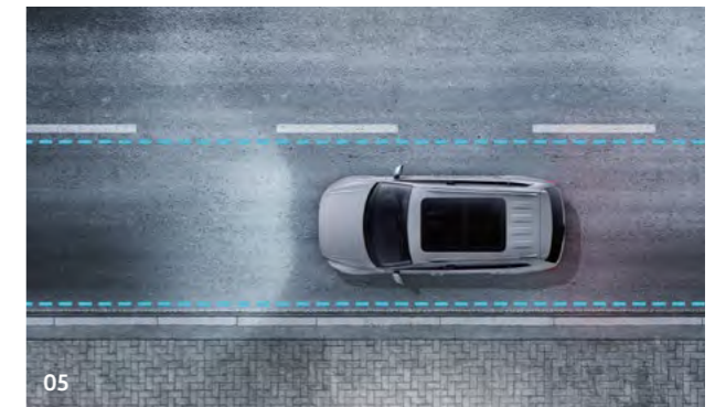
05 Lane Assist is a camera controlled warning system that warns you if your vehicle drifts out of its lane helping to reduce the chance of an accident and helping to make long motorway journeys safer. Using a camera located in the rear-view mirror unit, it monitors the road markings and prevents unintentional lane deviations. The system only intervenes if the indicators are not used, so if you decide to change lanes and indicate, the intelligent system recognises this and switches off. Standard on all models.
