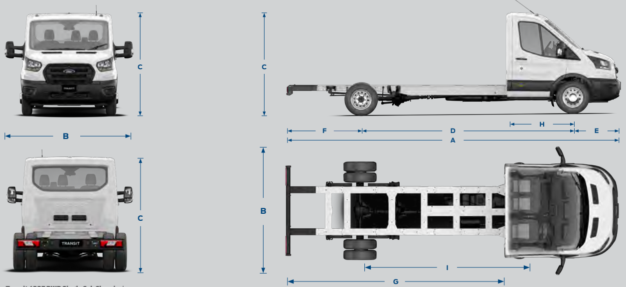
Transit 430E RWD Single Cab Chassis shown.
