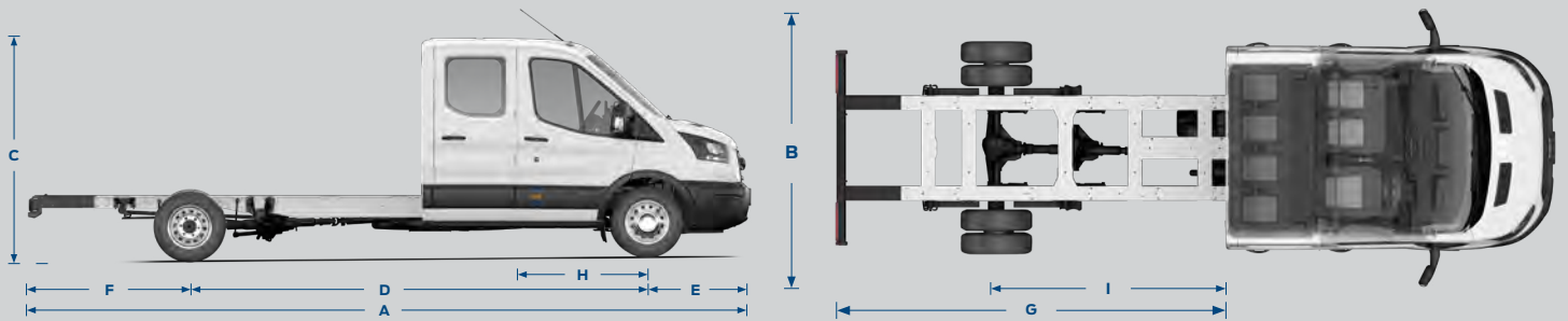
Transit 470E RWD Double Cab Chassis shown.
