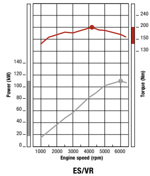
2.0L MIVEC DOHC Engine
