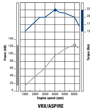
2.4L MIVEC DOHC Engine
