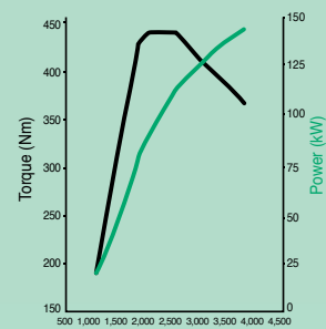
2.2 E-VGT Diesel Engine
