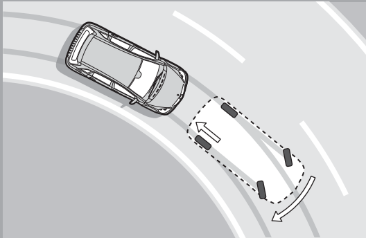
ESP®: brake application in the event of understeer
