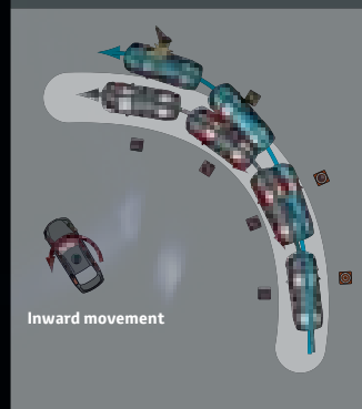
Front wheel skid control Vehicle Stability Control (VSC)
