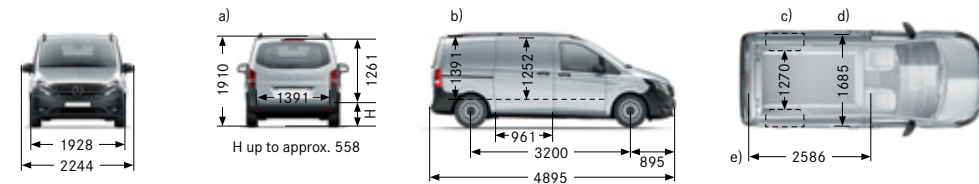
SWB panel van with 3200 mm wheelbase
