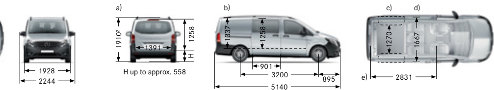
MWB Crew Cab with 3200 mm wheelbase
