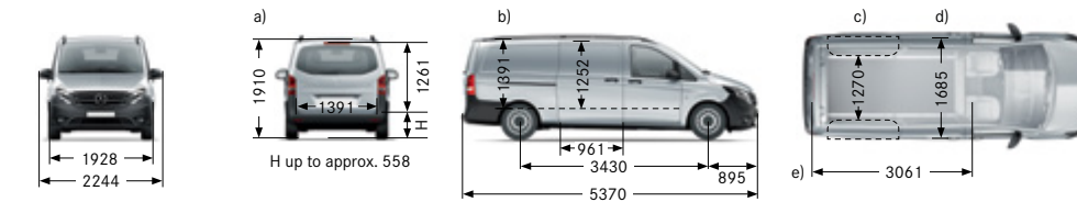
LWB panel van with 3430 mm wheelbase
