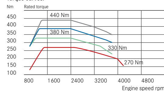
Torque curves:
