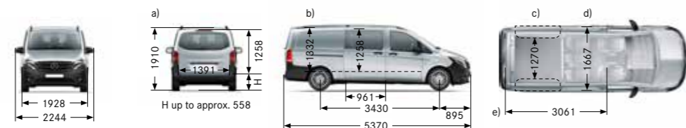
LWB Crew Cab with 3430 mm wheelbase
