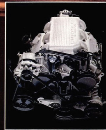
The 3.0-liter V-6 engine from Chrysler Motors and Mitsubishi Motors Corporation. A powerful addition to your Voyager when the going gets tough, the 3.0-liter V-6 features a dual-tuned intake manifold, overhead camshafts, and multipoint electronic fuel injection.
