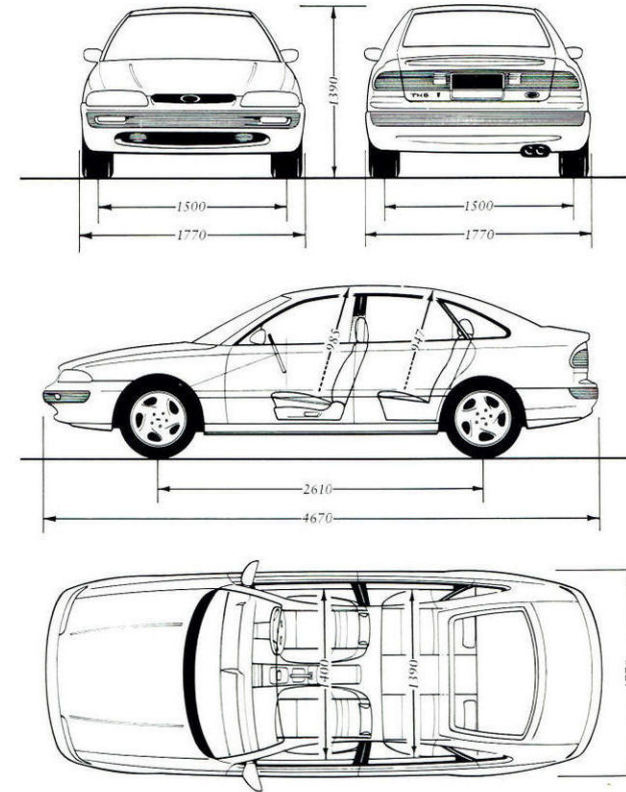
All dimensions are shown in (mm).
