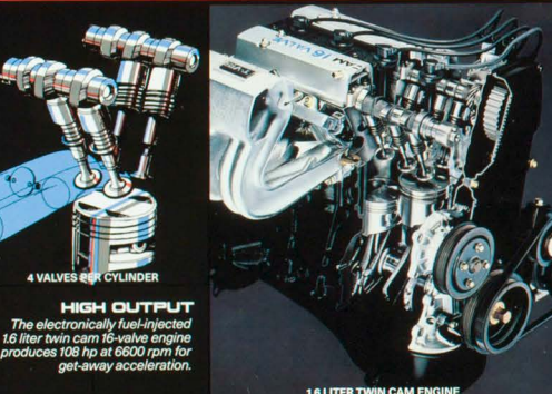
1.6 LITER TWIN CAM ENGINE
