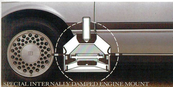
SPECIAL INTERNALLY DAMPED ENGINE MOUNT
