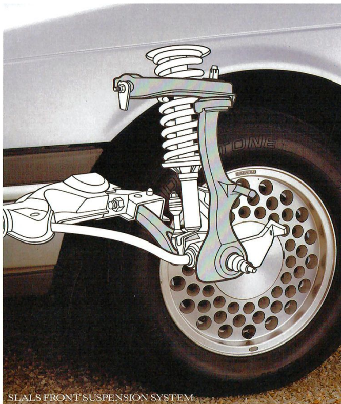
SLALS FRONT SUSPENSION SYSTEM
