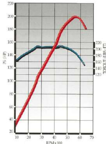
WITH 200 HP AND 210 LBS.-FT. OF TORQUE, THE 24-VALVE V-6 ENGINE PROVIDES EXCEPTIONAL PERFORMANCE AND DRIVEABILITY.
