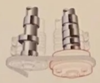
A Dual Overhead Camshaft (DOHC) and 4 valves per cylinder allow air and fuel to flow more efficiently. To give you even more power at both low and high rpm, the i-VTEC™ allows valve lift and timing by switching between two different sets of camshaft lobes.
