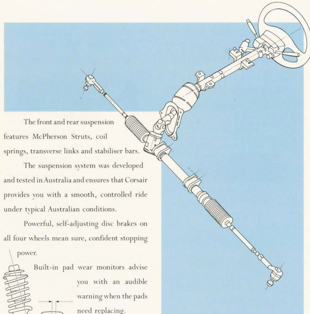
The precise rack-and-pinion steering system also features a tilt-adjust steering column.
