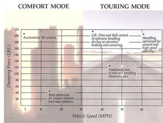
CORRELATION BETWEEN SUSPENSION FIRMNESS AND VEHICLE SPEED.
