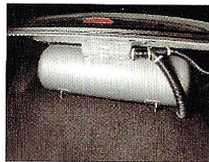
Specially designed LPG tank, fitted so that loss of boot space is kept to a minimum.
